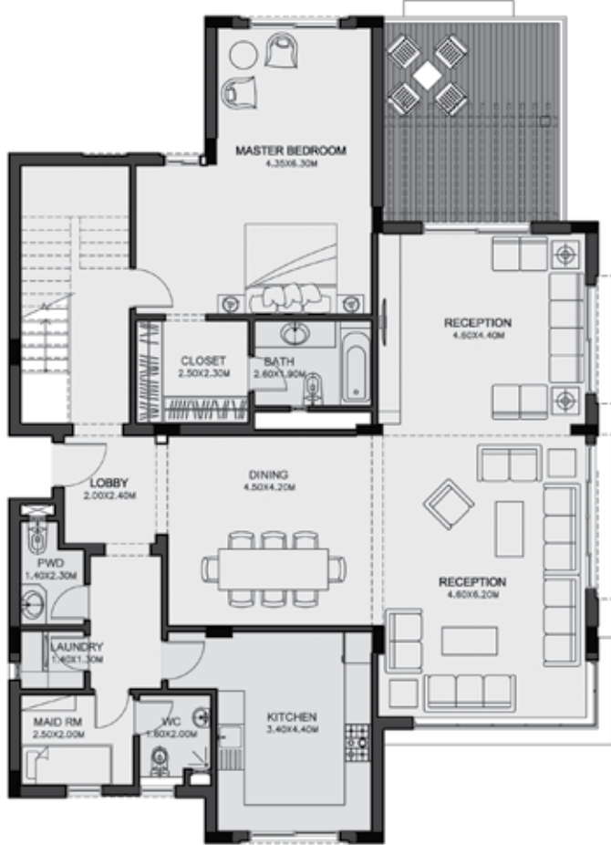
ENTRY LEVEL PLAN
